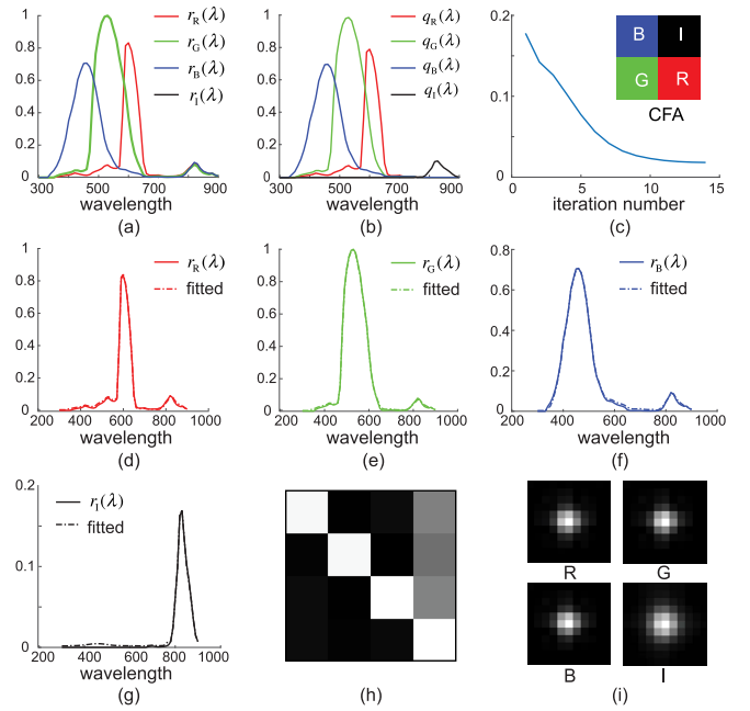
Fig. 1. (a) Measured spectral response of the OmniVision OV4682 sensor. (b) Optimized, ideal narrow-band spectral responses. Note that the crosstalk in the IR range is eliminated. (c) Convergence plot of the crosstalk matrix estimation. (d)–(g) are the R, G, B, I spectral response \mathbf{R} , and the fitted results \mathbf{C} * \mathbf{Q} at the estimated crosstalk matrix \mathbf{C} . (h) Estimated crosstalk matrix \mathbf{C} , corresponding to (b). (i) Calibrated point spread functions for all channels.
