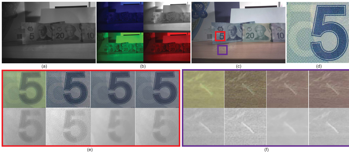
Fig. 8. Indoor scene without structured illumination. (a) Captured raw image, (b) extracted color channels, (c) the reconstructed RGB image of the proposed method. (d) Cropped photography of the figure 5 on the bill. We compare reconstructions with bilinear upsampling, Martinello et al. , Tang et al. and the proposed approach. In each close-up in (e) and (f), the figures we show are bilinear upsampling (first column), Martinello et al. (second column), Tang et al. (third column), and the proposed method (fourth column) of RGB (first row) and NIR (second row) channel respectively.
