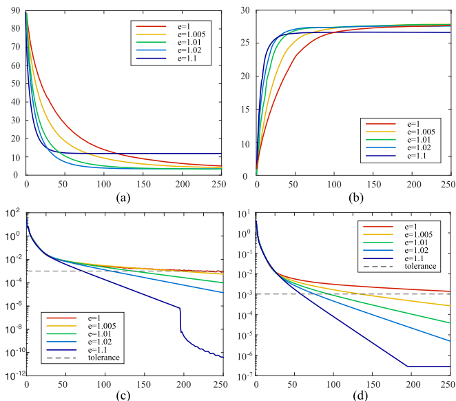
Fig. 6. Analysis of the step size e in Algorithm 1. We process the flower scene from Fig. 3(a) here and show: (a) the objective values, (b) PSNR, and the \ell_2 -norm of the primal (c) and dual (d) residuals [42].
