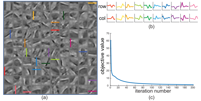
Fig. 2. (a) Learned convolutional kernels. (b) Horizontal and vertical scanlines picked from the dictionaries in (a). (c) Convergence plot of the learning procedure, showing a monotonically-decreasing decay.
